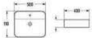
C000-78574(50)MP 500x400x110mm
