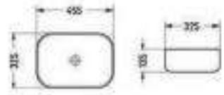
C000-78105MH
