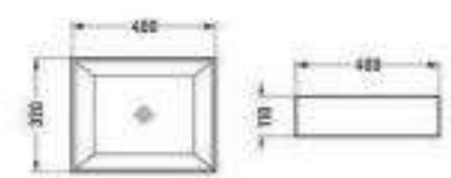
C000-78570B(40)MH 400x320x110mm
