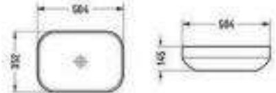
C000-78589MDB
